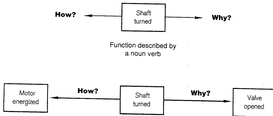
Figure 3.11 Building a FAST diagram.
