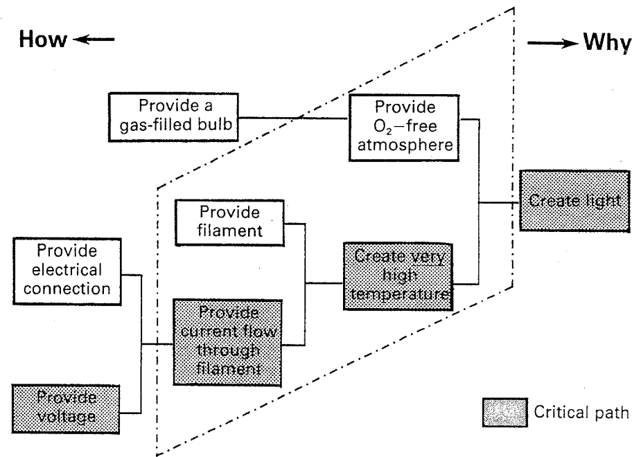
Figure 3.12 The FAST diagram for the light bulb showing critical path and boundaries.
